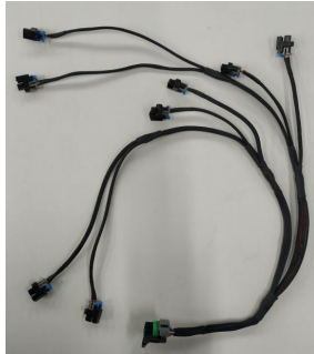
132. 8 cyl universal fuel injection wire harness- with EV6 Injector Connector
