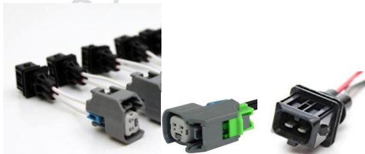
130. Injector conversion adapter harness - uscar EV6 EV14 harness To Denso Fuel Injector
