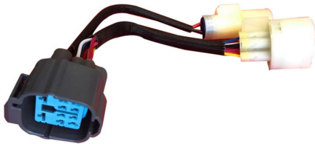
112. Distributor Adapter Harness OBD0 to OBD2 10 Pin Honda Conversion Jumper
