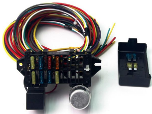
17. 12 circuit universal hot rod wiring harness
