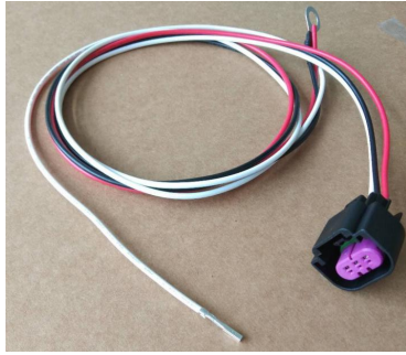
122. GM E85 Flex Fuel Sensor Connector Wire Harness Pigtail 12 inches wires
