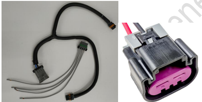
16. 8 circuit universal hot rod wiring harness
