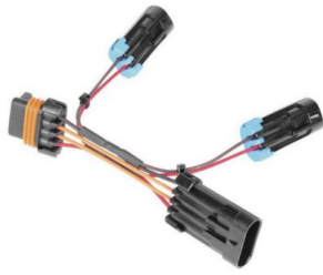
56. POLARIS T-Map Sensor Repair Pigtail Harness Sportsman RZR Ranger -12 inches
