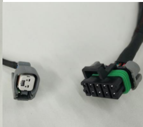
133. 8 cyl universal fuel injection wire harness- with EV1 Injector Connector
